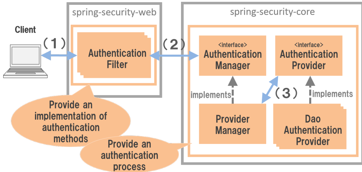
Figure.9.2 Authentication process architecture
