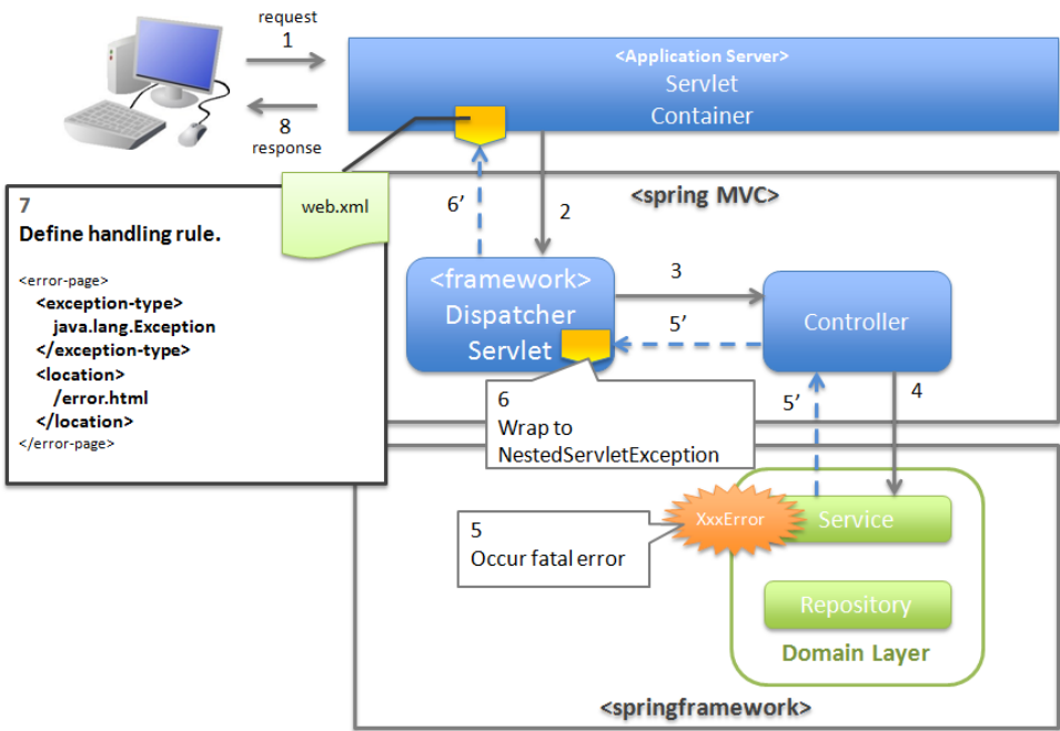
Figure.4.7 Figure - Handling method when a fatal error has been detected
