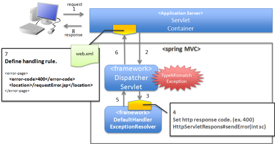
Figure.4.6 Figure - Handling method when notifying that the request contents are invalid
