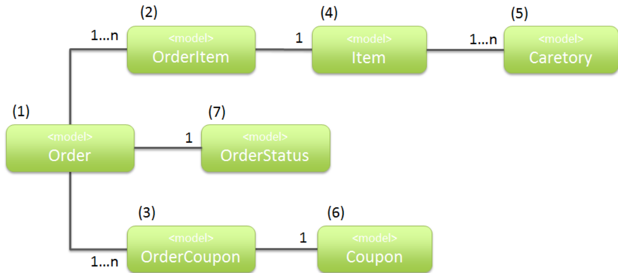
Figure.6.7 Picture - Class(JavaBean) diagram
