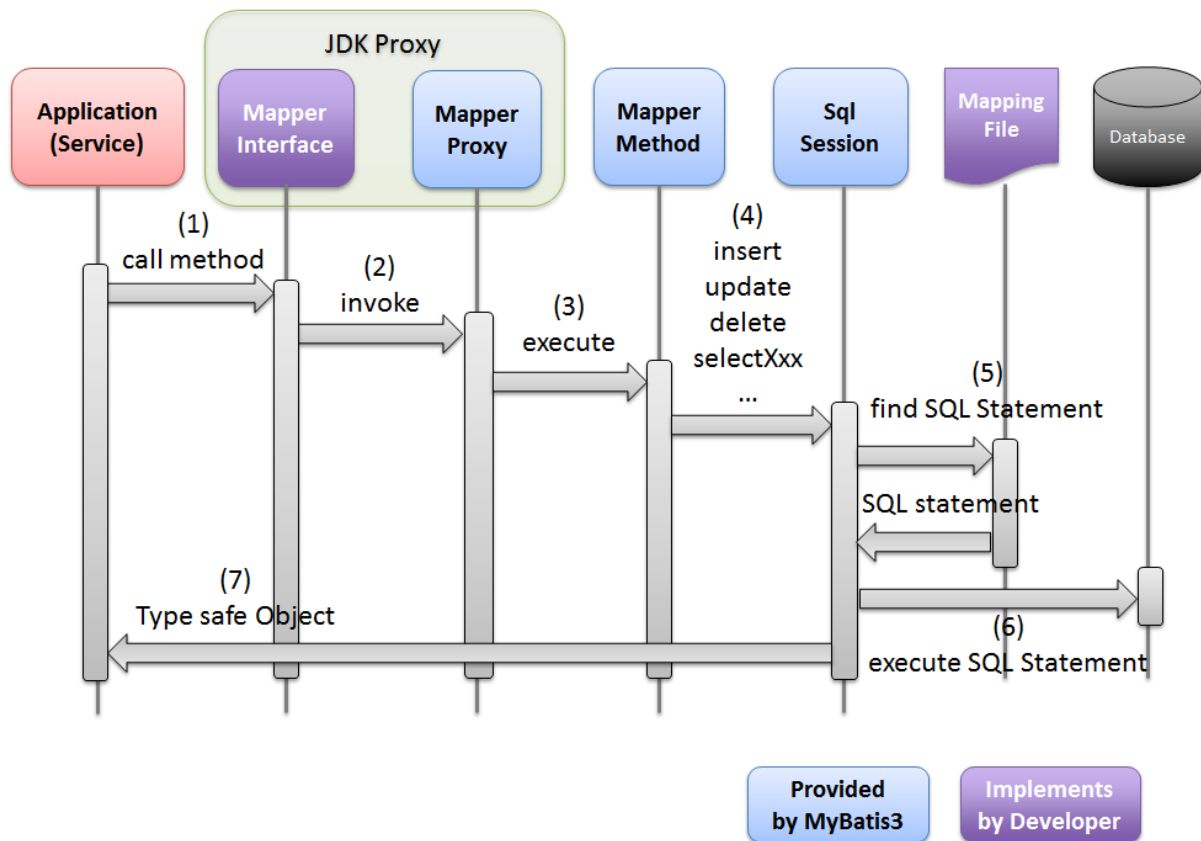
Figure.6.5 Picture - Mapper mechanism
