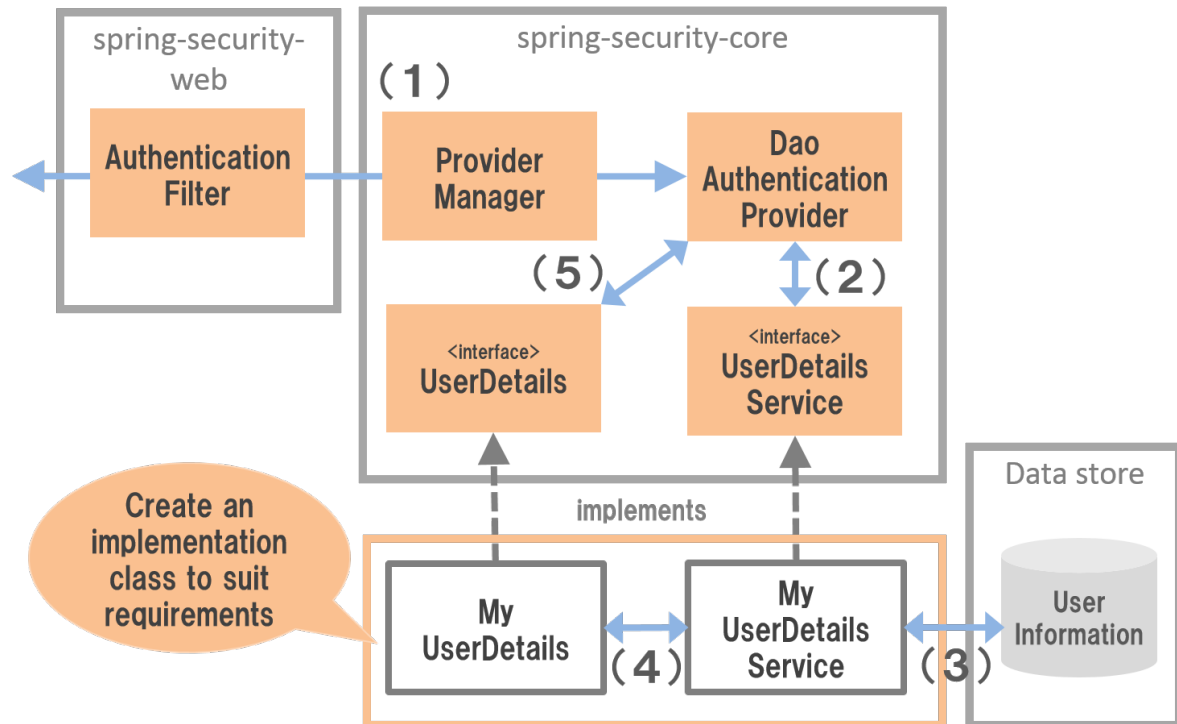
Figure.9.4 DB authentication system
