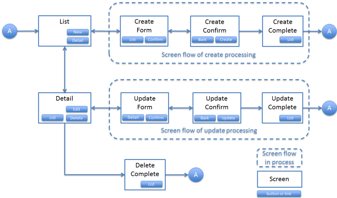
Figure.3.2 Picture - Screen flow of entity management function
