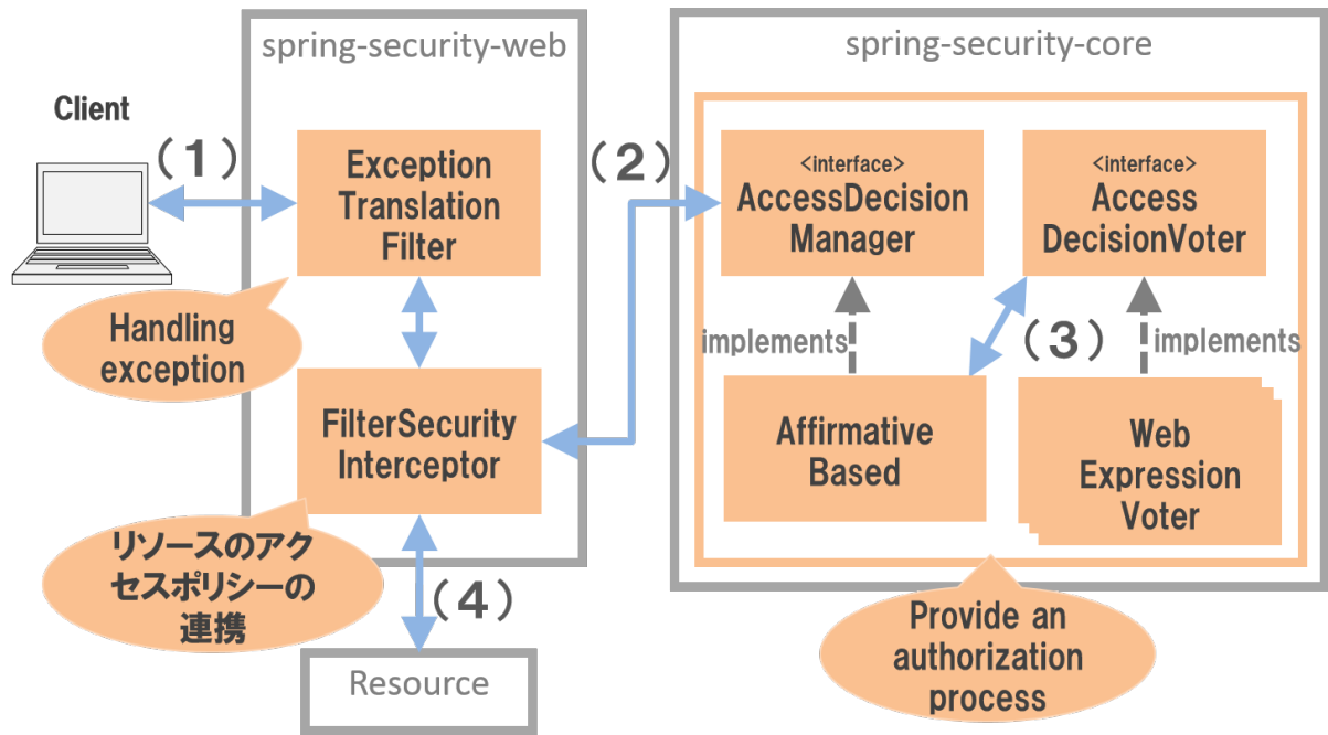
Figure.9.7 Authorization process architecture
