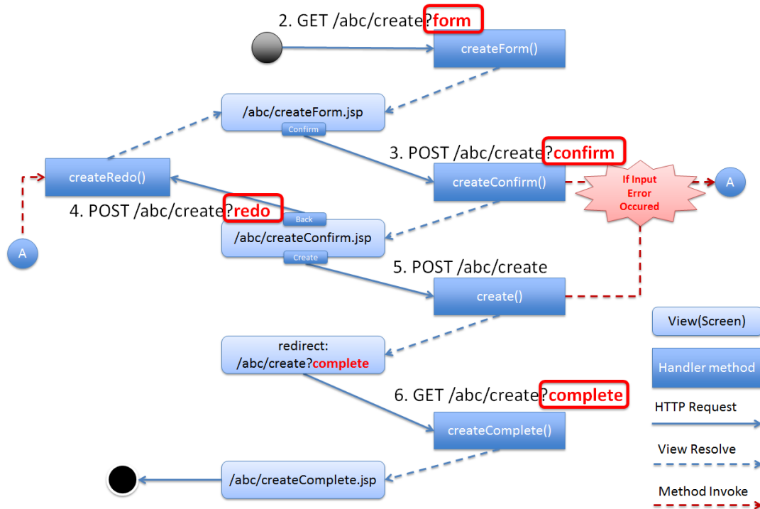
Figure.3.4 Picture - Request flow of entity create processing
