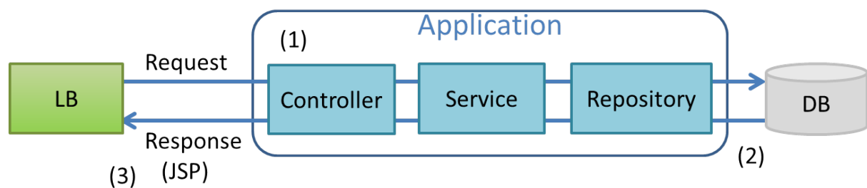
Figure.4.25 Picture - HealthCheck Configuration
