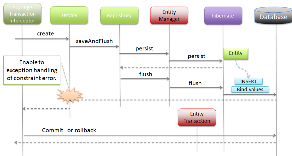
Figure.6.27 Picture - Sequence of persistence processing when flush method is used
