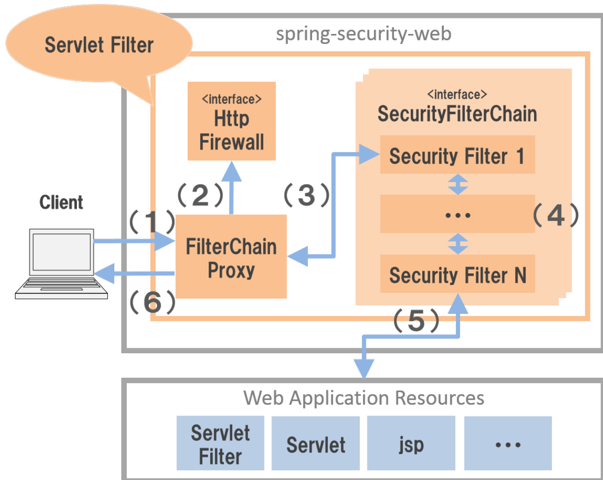
Figure.9.1 Spring Security Framework architecture
