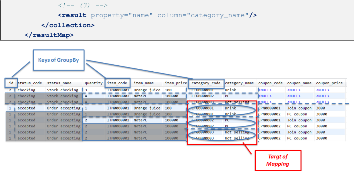
Figure.6.13 Picture - resultMap for Category
